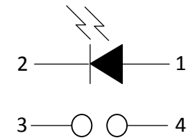
LED Schematic
