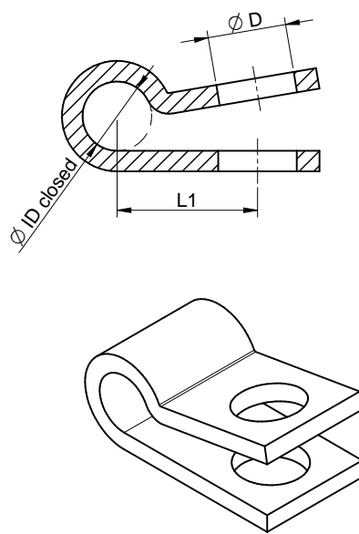
sectional drawing A-A
