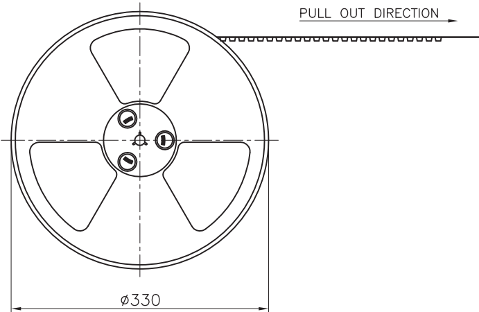
TAPE PACKING
