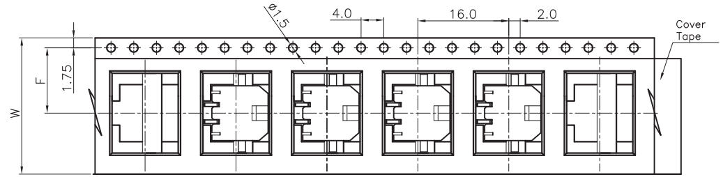
Pull Out Direction For Reel width (dimension W)24mm Single row hole
