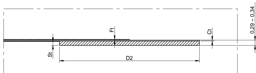
Detail C
