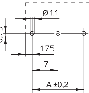
PCB LAYOUT - COMPONENT VIEW
