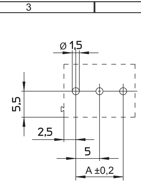
PCB LAYOUT - COMPONENT VIEW
