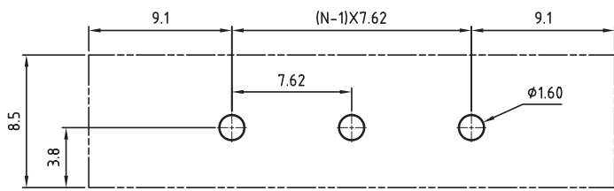
PCB LAYOUT - COMPONENT VIEW
