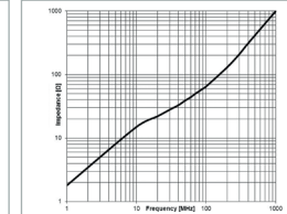
7427218 Pins 30 Adh. Tape T-SH60081242 Material 4W620
