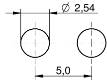
MOUNTING HOLES
