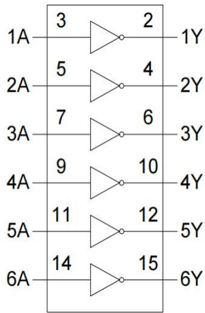
Figure 1. Functional symbol
