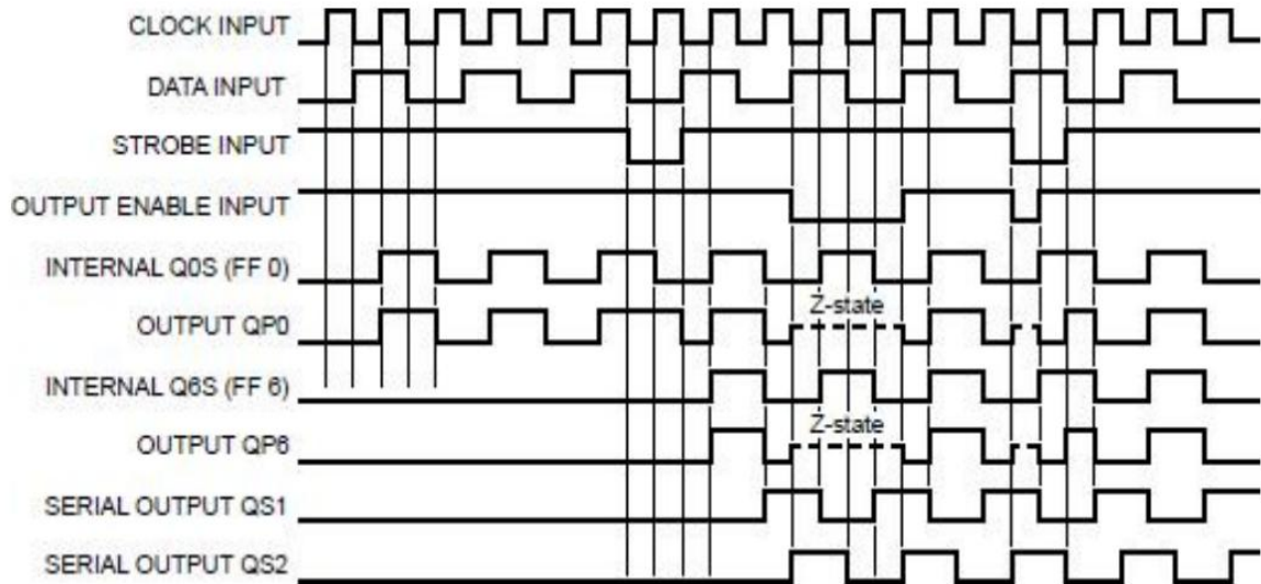
Figure 4. Timing diagram
