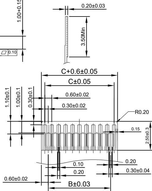
Applicable FPC
