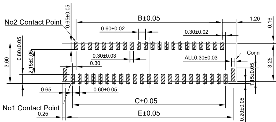
FPC/FFC Insert Direction Recommended P.C.B Layout
