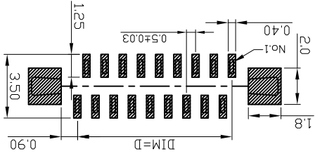
RECOMMENDED PC BOARD LAYOUT (ALL TOLERANCE ARE ±0.05)
