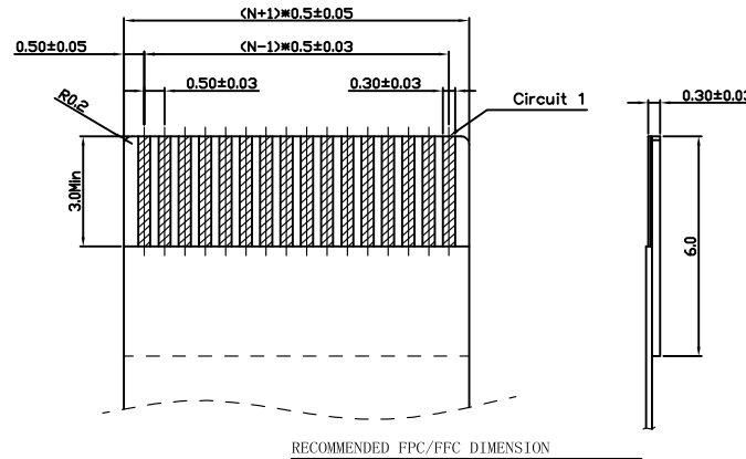
RECOMMENDED FPC/FFC DIMENSION
