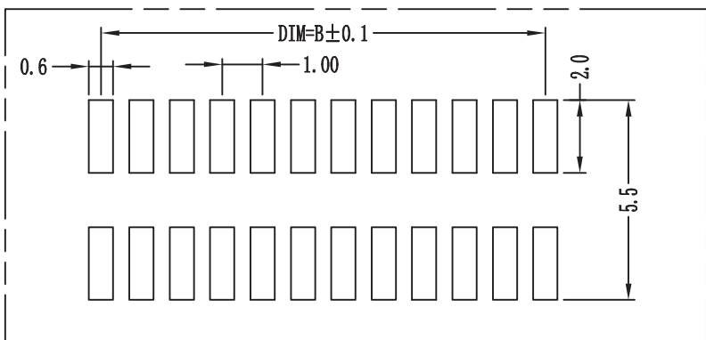
PCB Layout
