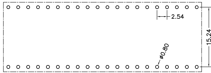
P. C. B LAYOUT
