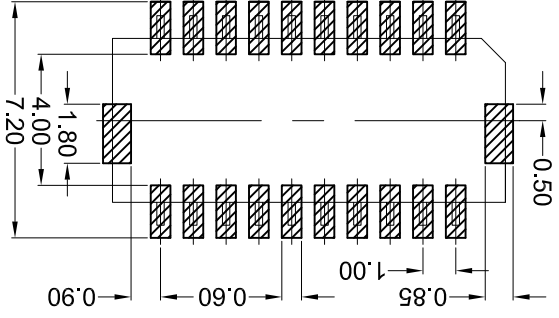
Recommend PCB Layout General Tolerance±0.05
