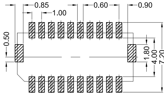
Recommand PCB Layout General Tolerance±0.05
