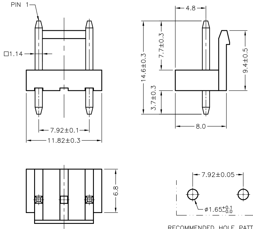
RECOMMENDED HOLE PATTERN
