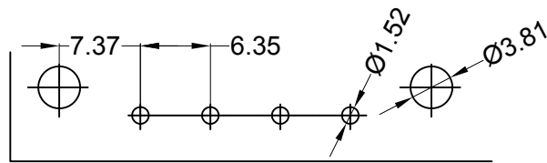
Recommended P.C.B Layout General Tolerance \pm 0.05
