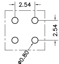
P. C. B LAYOUT
