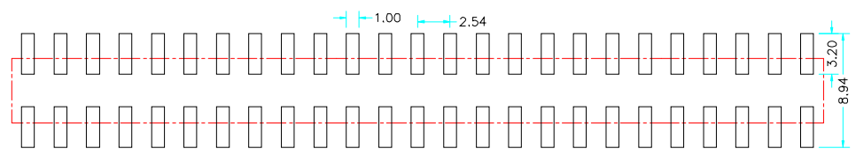
P. C. B LAYOUT
