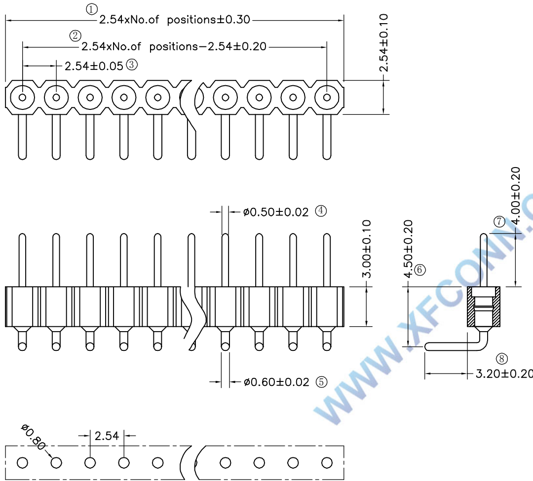
P. C. B LAYOUT
