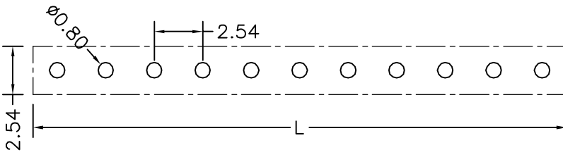
P. C. B LAYOUT
