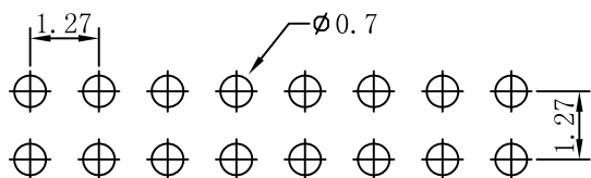
PCB LAYOUT
