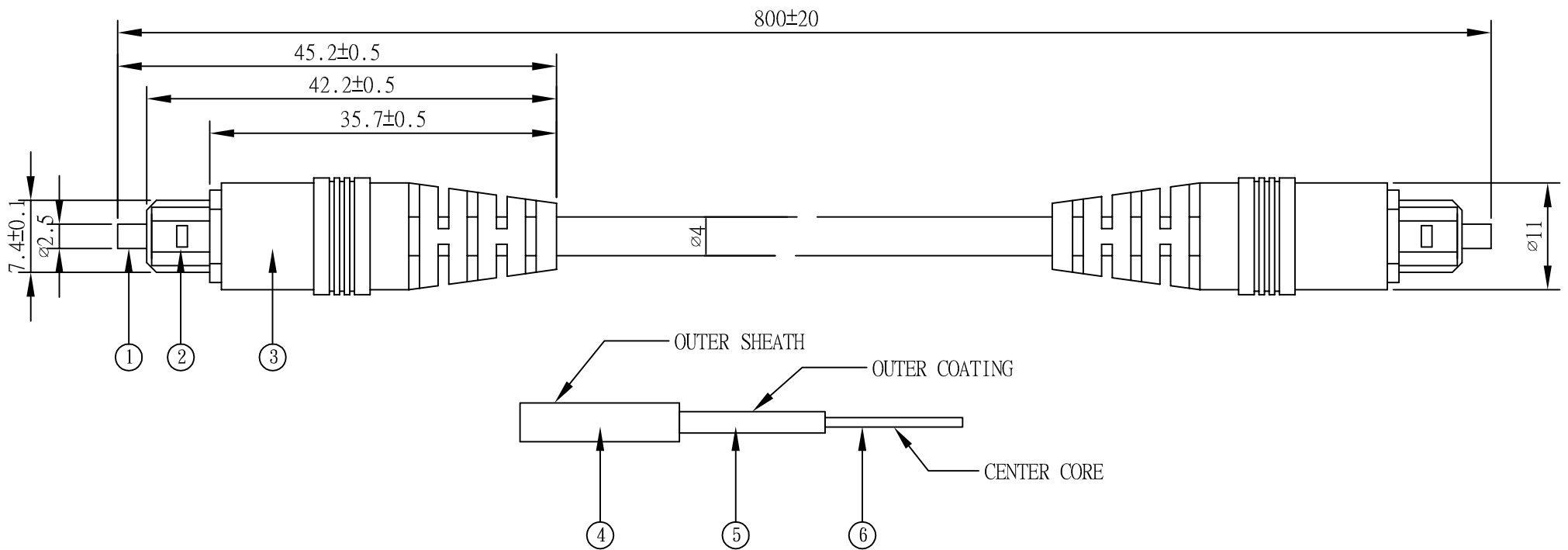
FIBER SPECIFICATION
