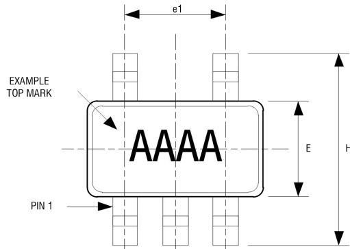
5LD SOT-23 PACKAGE OUTLINE DIMENSIONS
