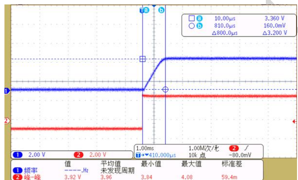
Enable Startup @ V_{OUT}=3.3V, I_{OUT}=0.8A
