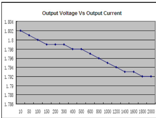
V_{in}=3.6V, V_{out}=1.8V
