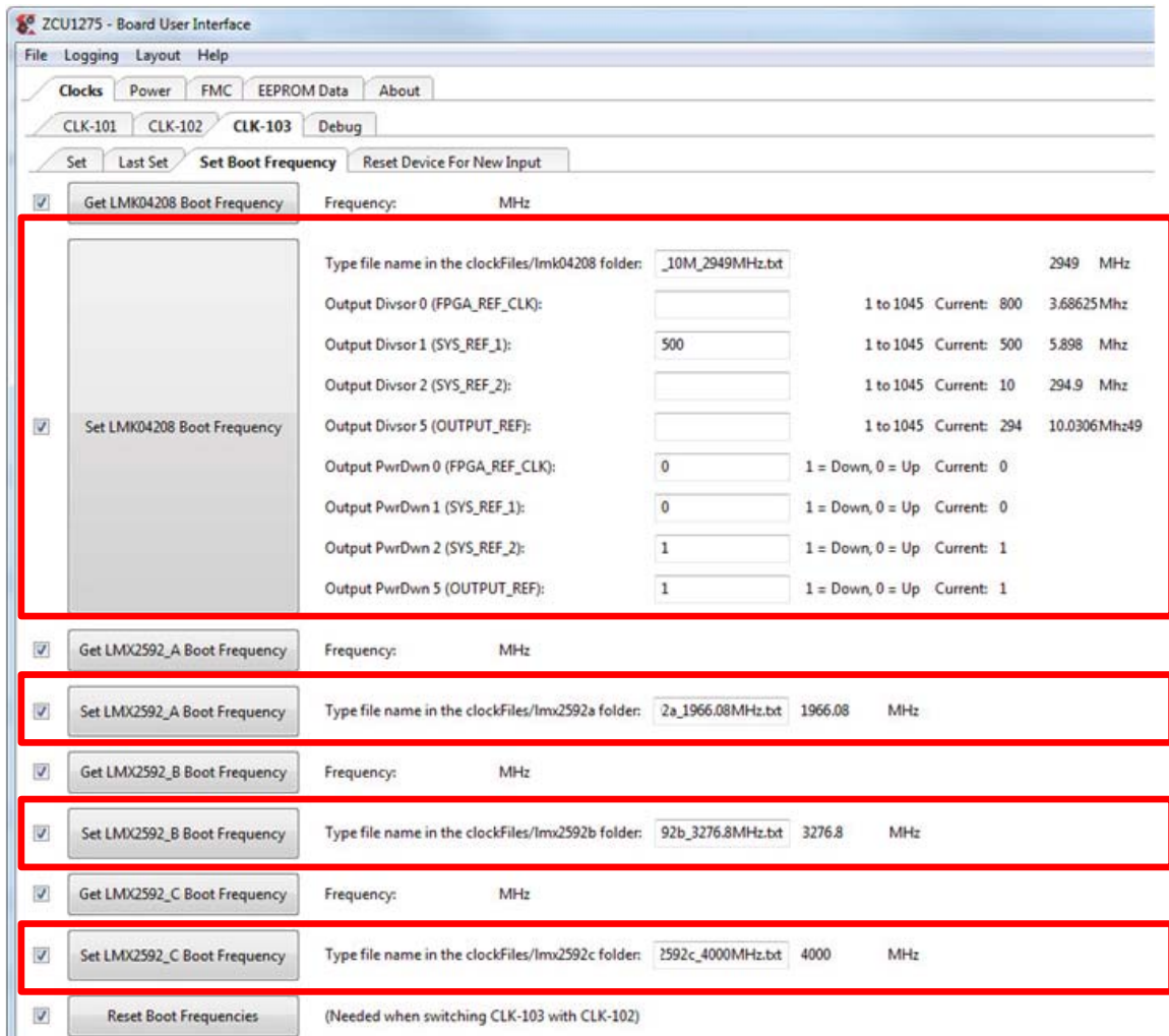
Figure D-15: CLK-103 Set Boot Frequency Tab
