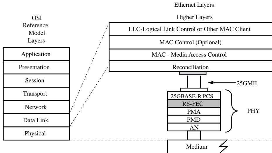
Figure 1: IEEE Std 802.3 Ethernet Model
