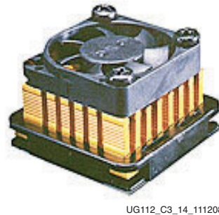
Figure 3-15: Example of Active Heatsink for BGA (Malico)
