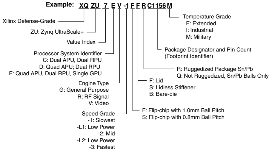
Figure 5: XQ Zynq UltraScale+ MPSoC and RFSoc Ordering Information
