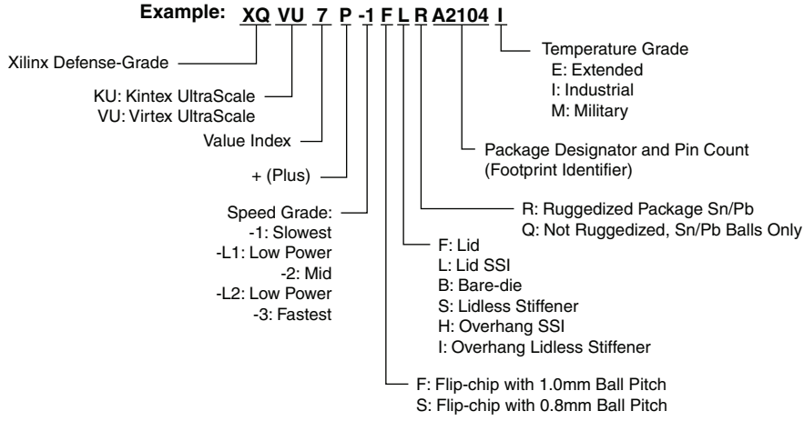
Figure 4: XQ UltraScale+ FPGA Ordering Information
