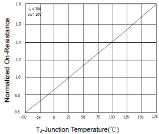
Figure 4 Rdson-Junction Temperature
