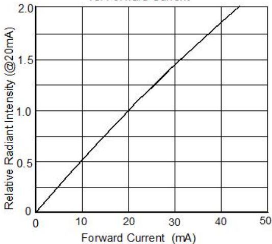
Fig.5 Relative Radiant Intensity vs. Forward Current
