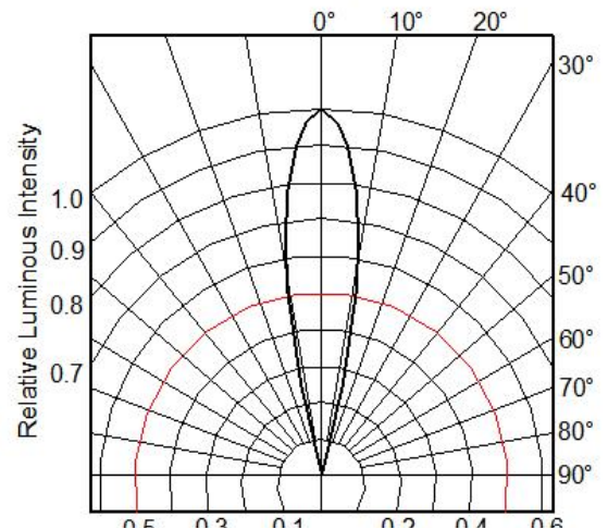
Fig.6 Radiation diagram(Ta=25°C)
