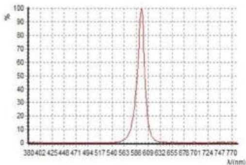
◆ 发射光谱(Emission spectrum)
