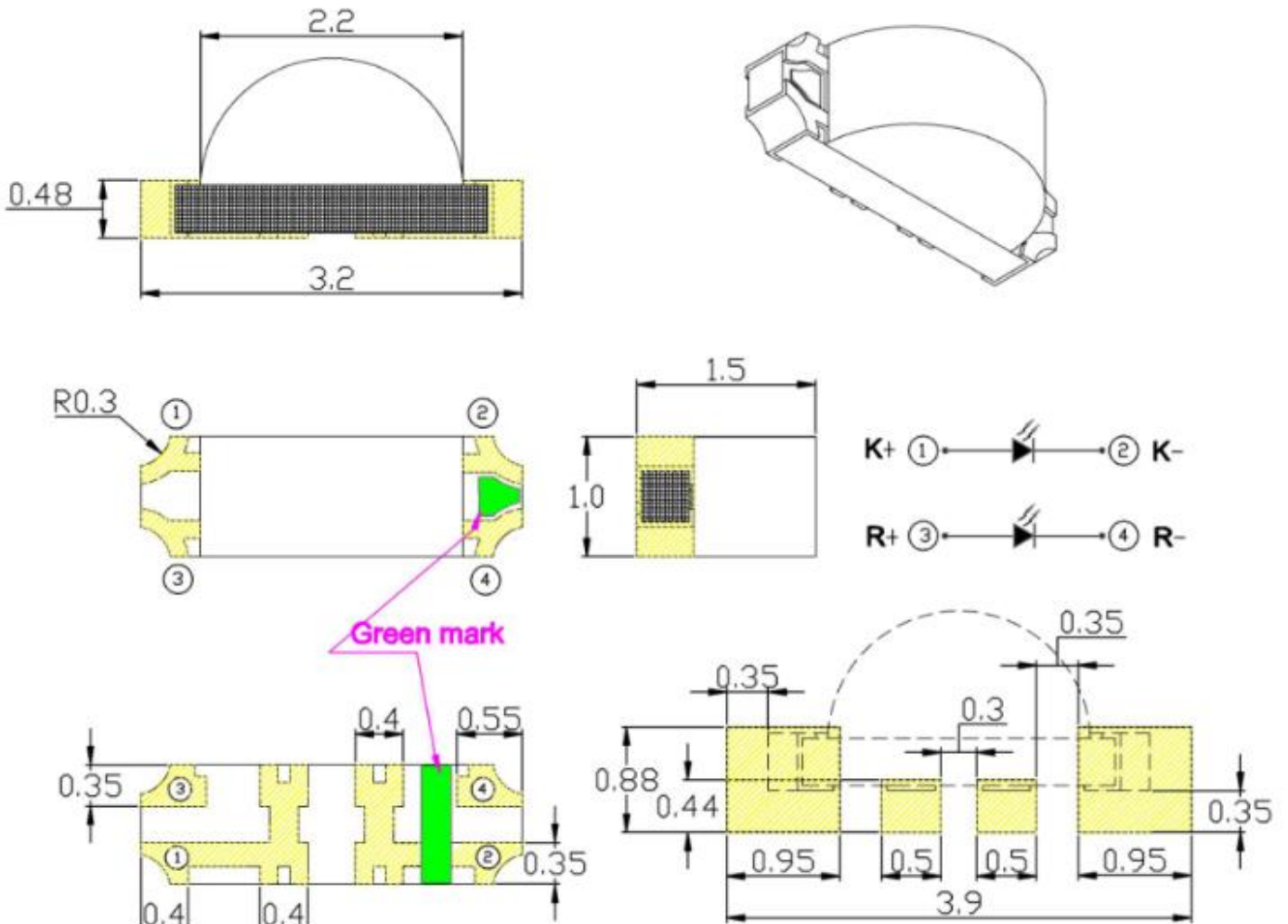
建议焊盘尺寸 Recommended pad size
