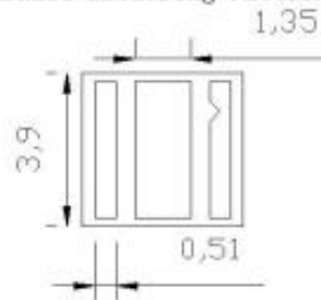
建议焊盘尺寸图 Recommended Soldering Pattern
