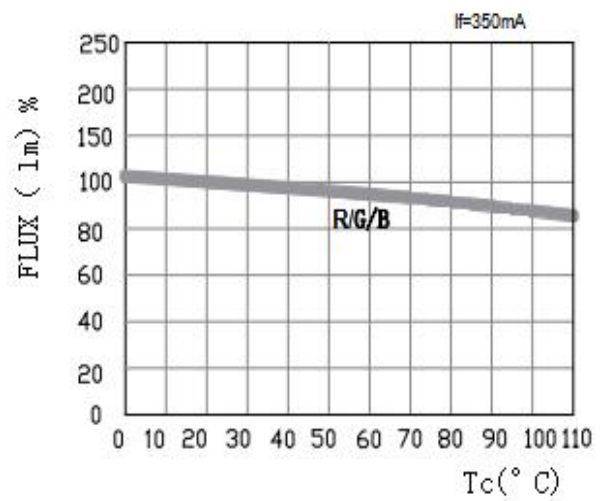
Temperature vs Relative Luminous Flux
