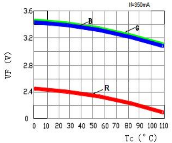
Temperature vs Forward Voltage
