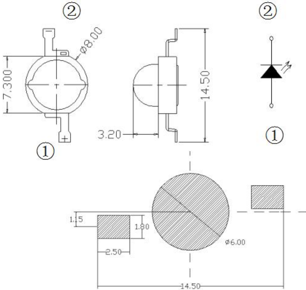
推荐焊盘 Recommand soldering pad
