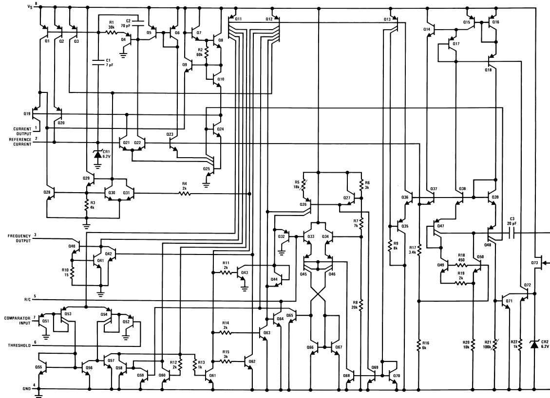
Schematic Diagram
