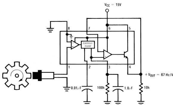
Minimum Component Tachometer Diagram
