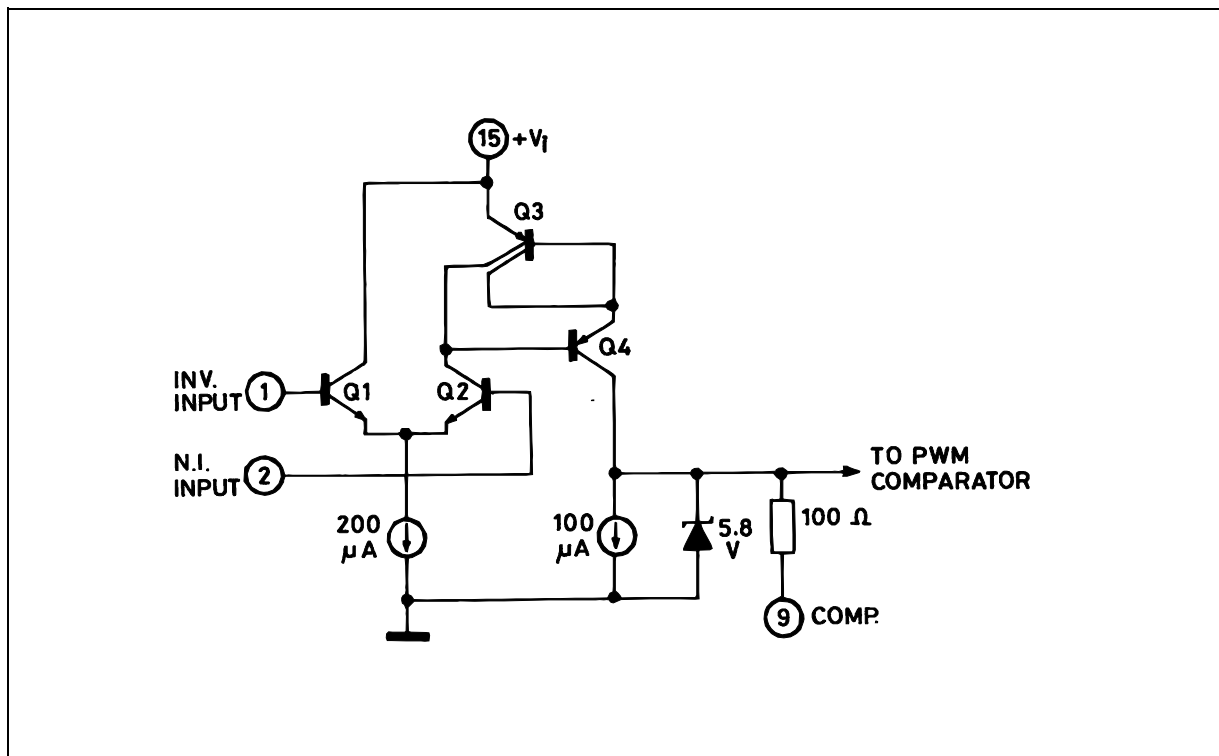
Figure 5 : Error Amplifier.
