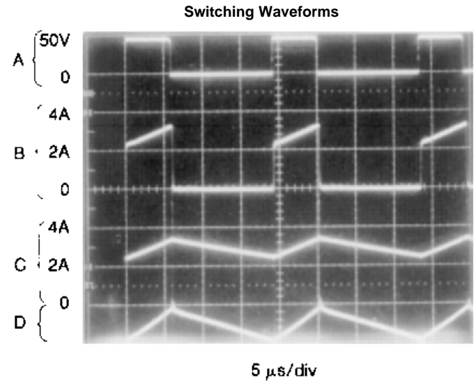
Figure 19. V_{OUT} = 15V A: Output Pin Voltage, 50V/div B: Output Pin Current, 2A/div C: Inductor Current, 2A/div D: Output Ripple Voltage, 50 mV/div, AC-Coupled Horizontal Time Base: 5 µs/div
