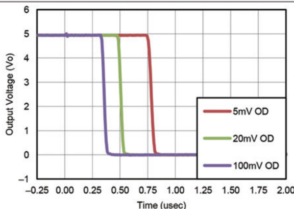
Figure 9. Response Time for Various Overdrives (Negative Transition)
