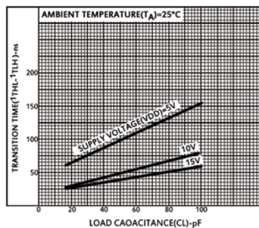
Fig.7- Typical Typical low-to-high transition time vs. load capacitance.
