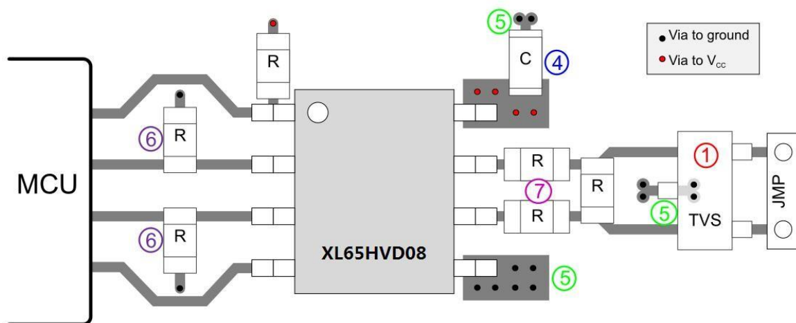
Figure 25.XL65HVD08 Layout example
