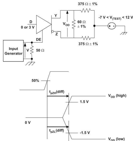
Figure 1. Driver Enable Time From DE to V_{OD}
