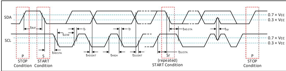
Figure 4. Definition of timing on the I 2 C-bus
